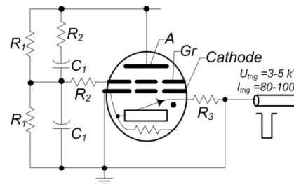
Fig. 3. Principal circuit of gradient grid feed.
